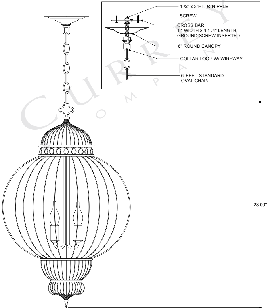
FRONT VIEW
