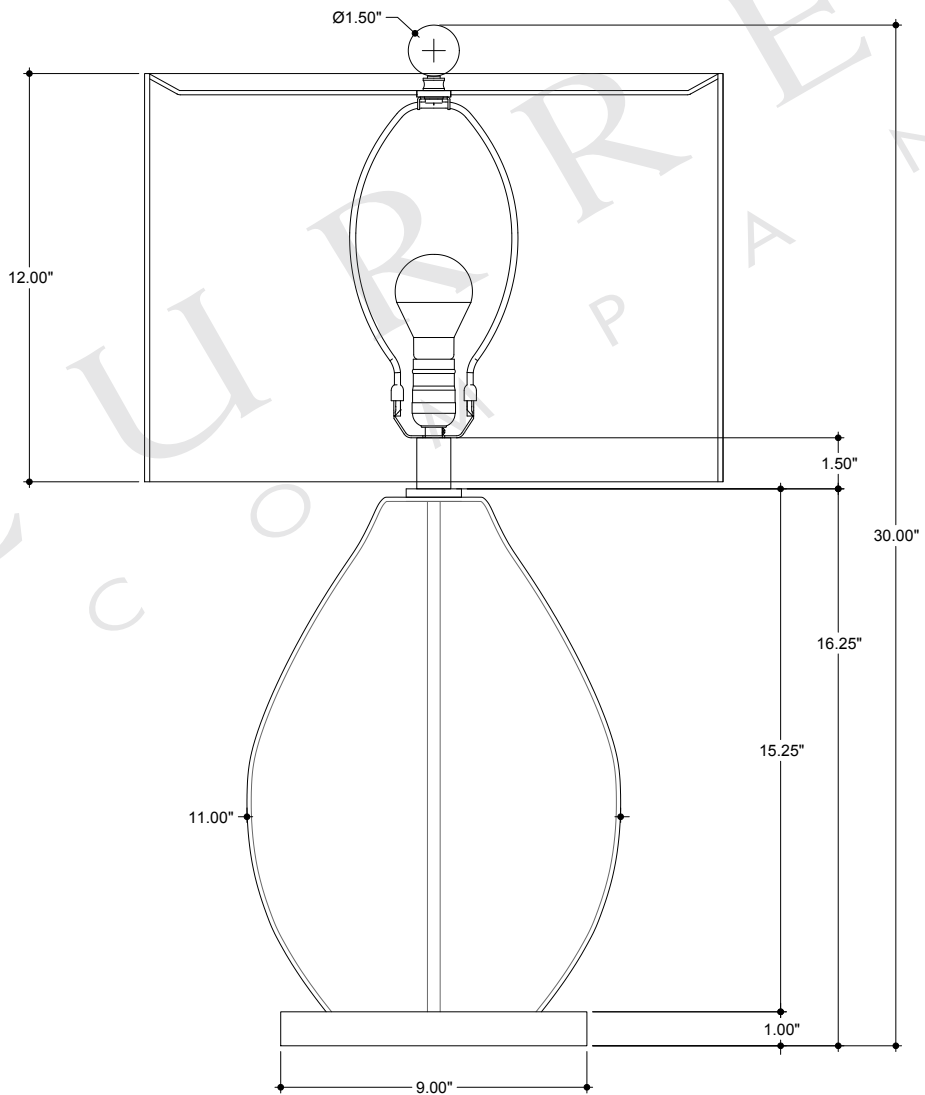
FRONT VIEW
