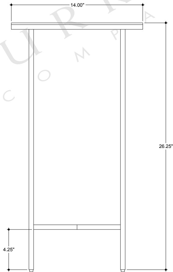
FRONT VIEW
